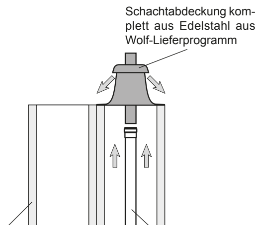
Schornstein T400
