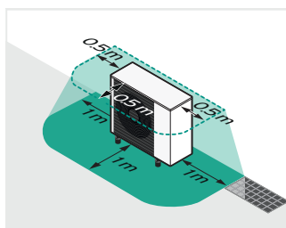
aroTHERM plus/6
