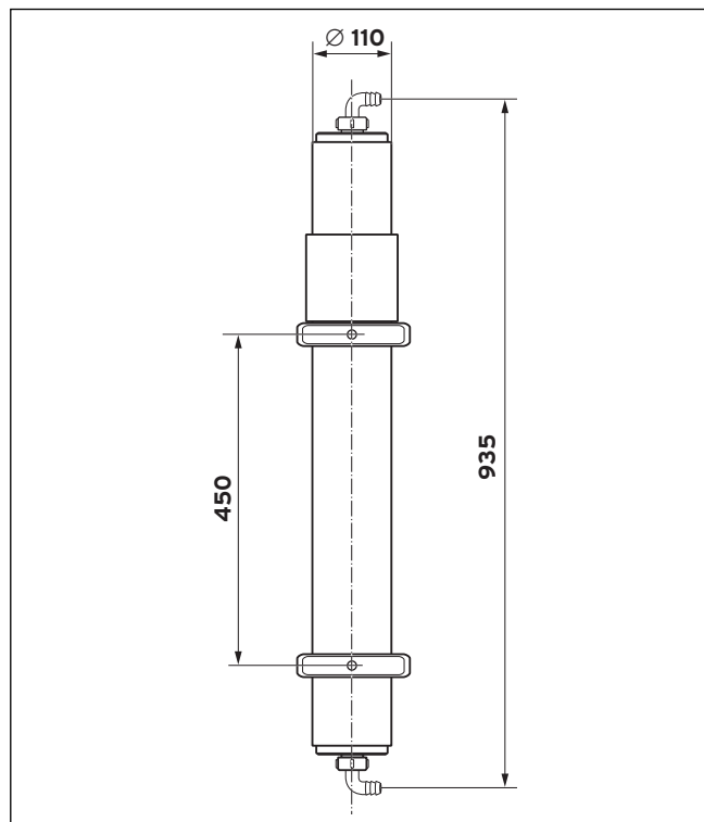
Fig. 3.1 Dimensions and installation
