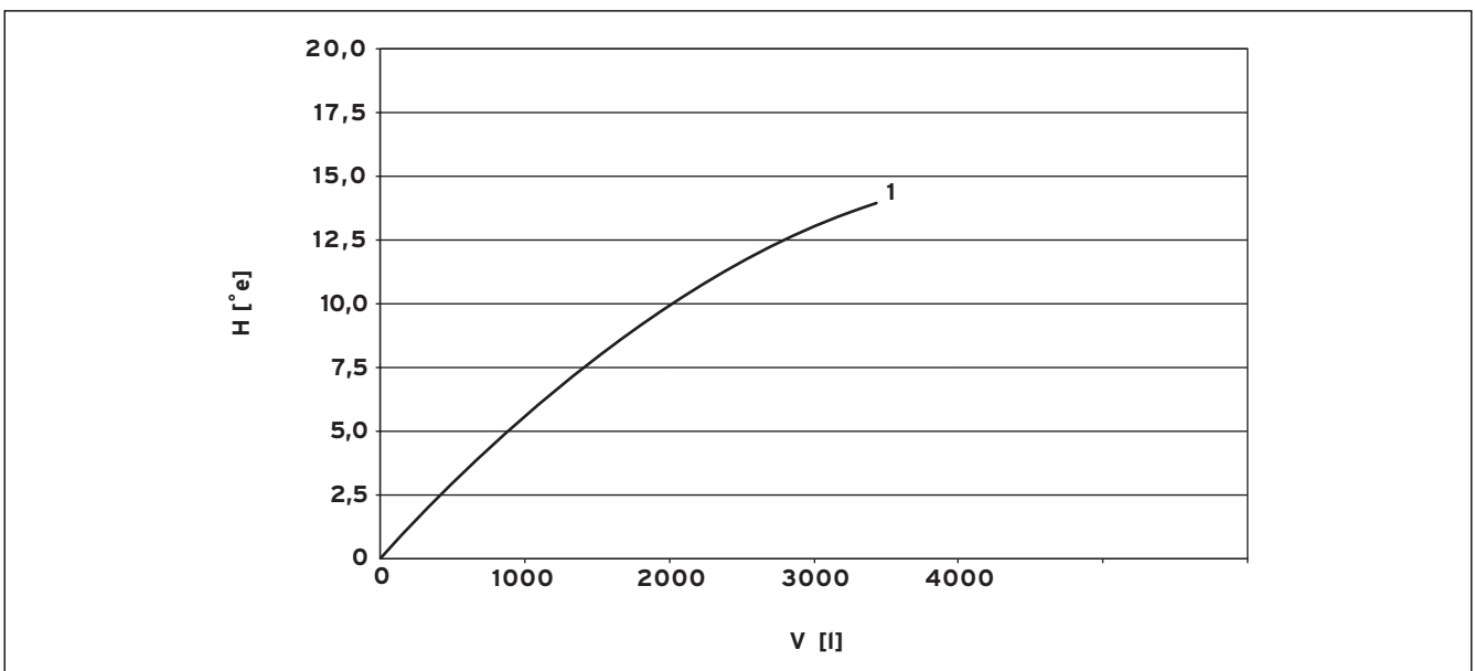
Fig. 4.2 Variation in hardness (carbonate hardness) of the filling water with respect to fill volume
