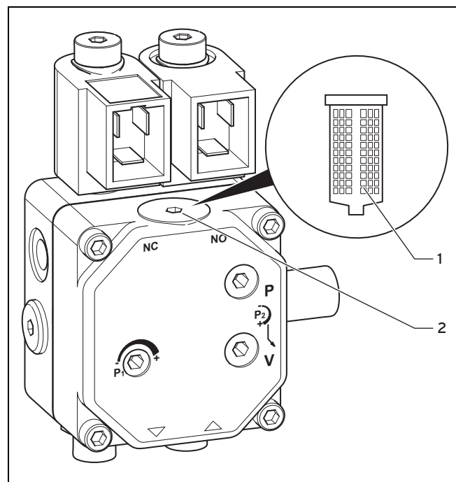
11.7: Ölpumpenfilter reinigen
