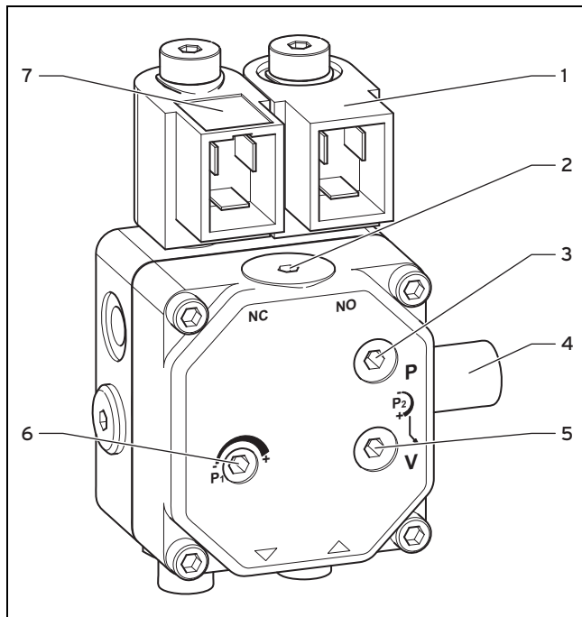
11.16: Ölpumpe
