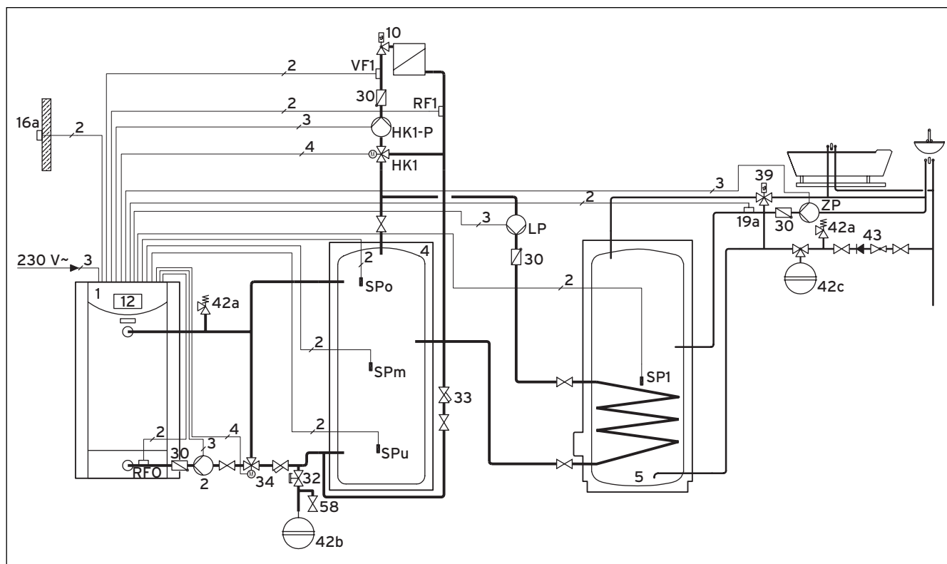
Abb. 6.15 Hydraulikplan 1
