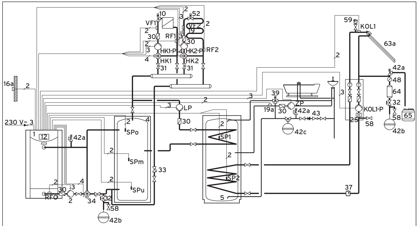
Abb. 6.17 Hydraulikplan 2
