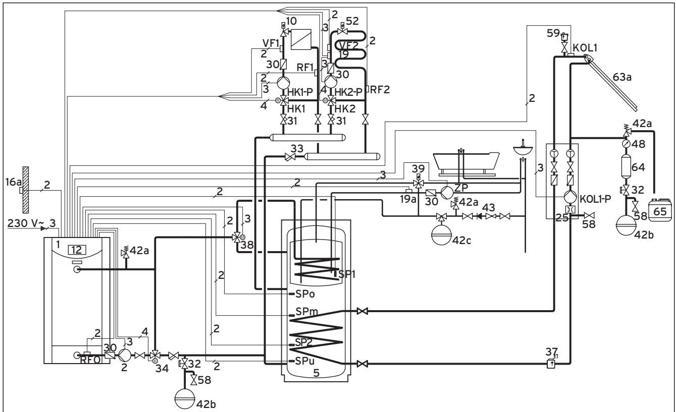
Abb. 6.19 Hydraulikplan 3
