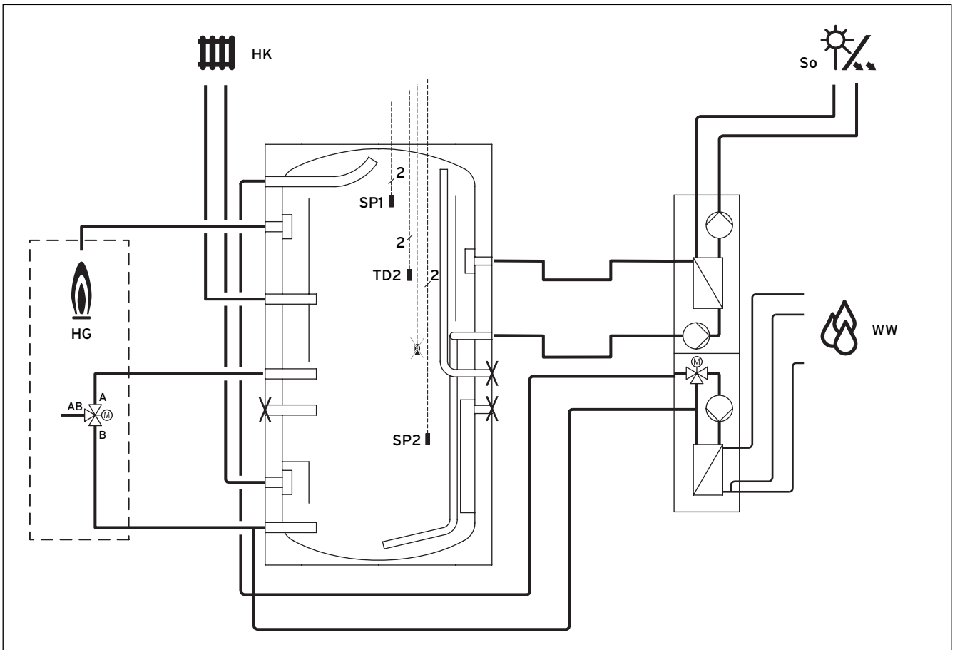
Abb. 3.15 Detail-Plan Wandmontage
