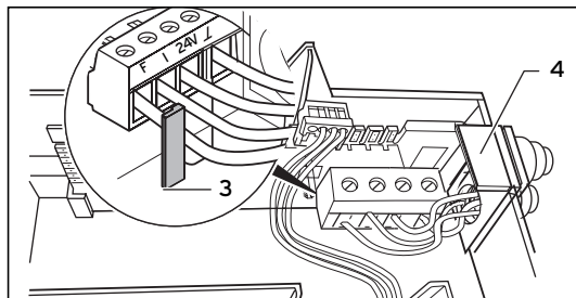
Fig. 4.3 Cable bushing
