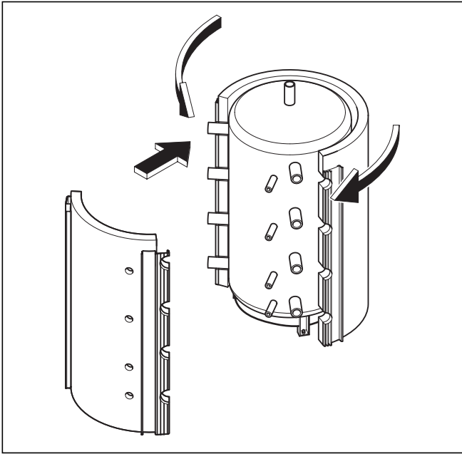
Fig. 4.8 Fitting the insulating jackets
