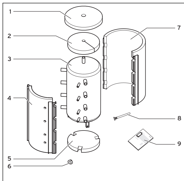
Fig. 4.1 Scope of delivery
