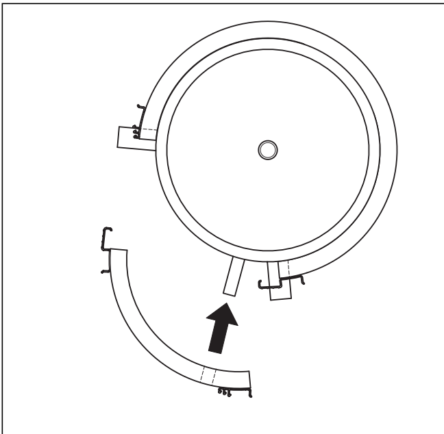
Fig. 4.9 Attaching the rear insulating jacket (from above)
