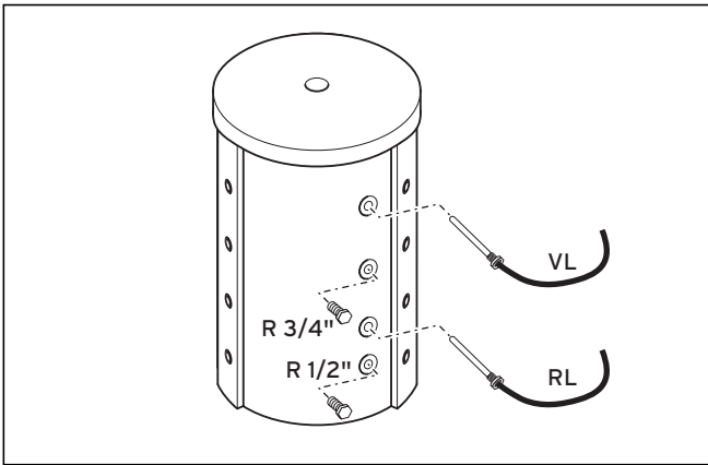
Fig. 5.2 Temperature sensor connections and plugs
