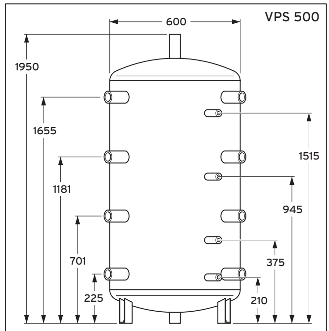
Fig. 4.3 VPS 500 dimensions *
