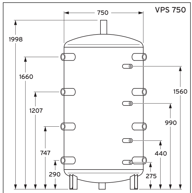
Fig. 4.4 VPS 750 dimensions *
