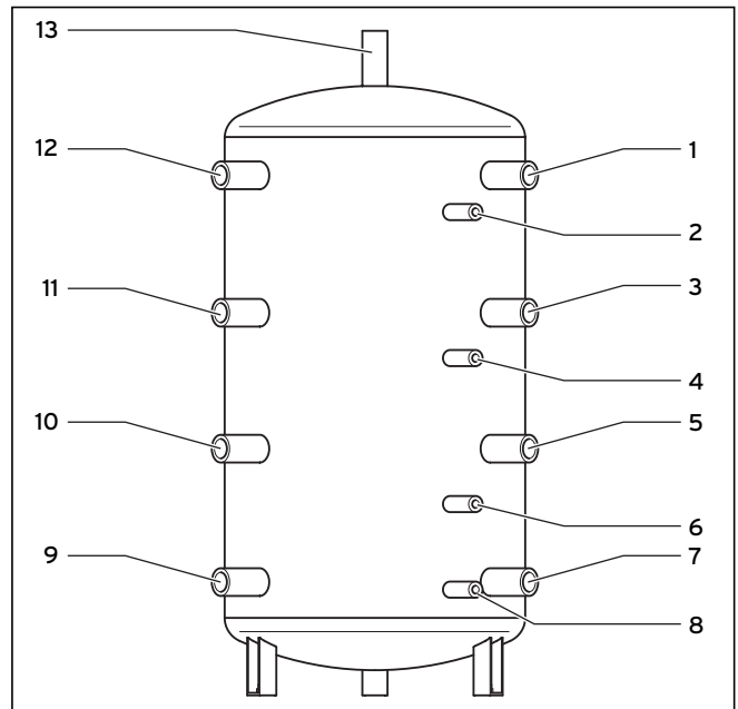
Fig. 2.2 Connections (rear)
