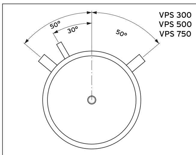
Fig. 4.5 Connection angles on the rear side (from above)
