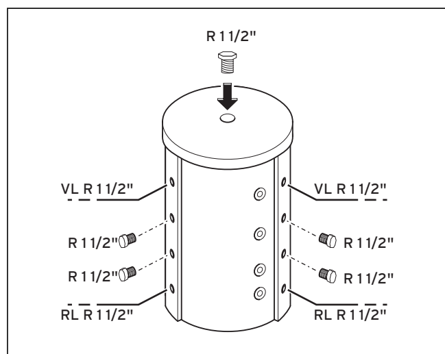
Fig. 5.1 Water connections and plugs
