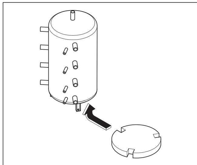
Fig. 4.7 Fitting the bottom pad
