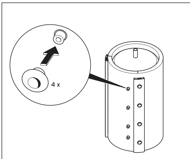
Fig. 4.12 Attaching the rosettes
