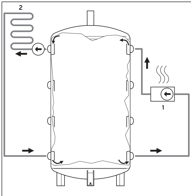
Fig. 2.1 Principle of operation of the buffer cylinder
