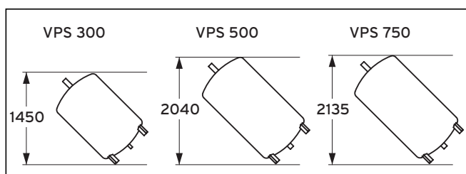
Fig. 4.6 Tilt measurement
