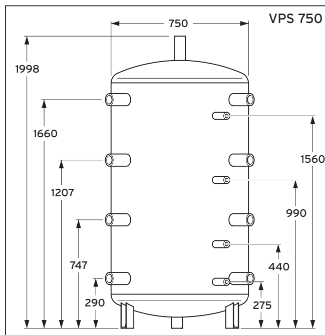
Fig. 4.4 Dimensions VPS 750 *
