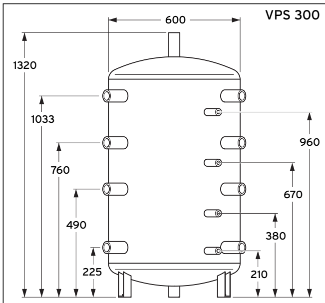
Fig. 4.2 VPS 300 dimensions *
