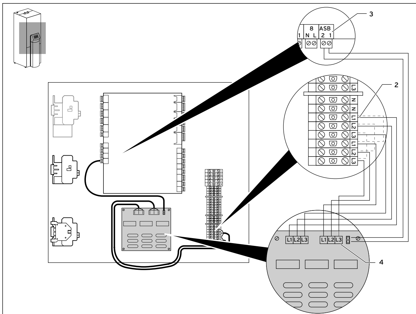
Fig. 4.6 Collegamento al geoTHERM VWS/VWW/VWL-S ..2 e VWS ..3
