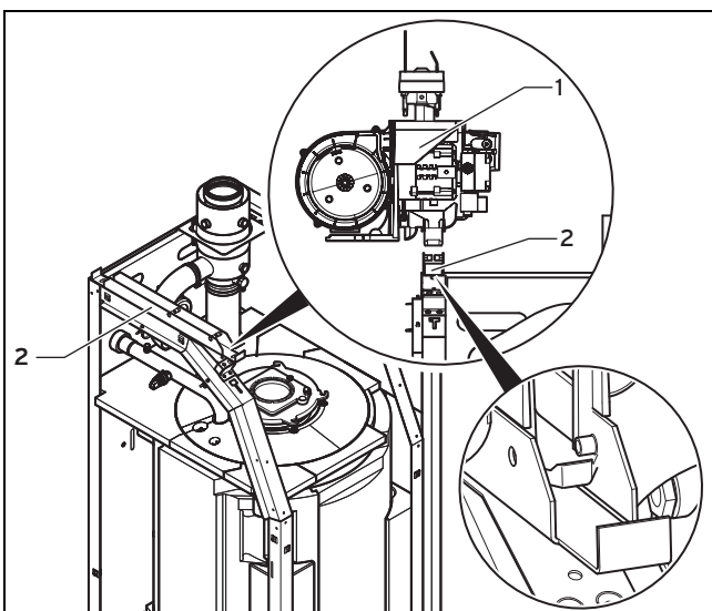
1 Brenner 2 Traverse
