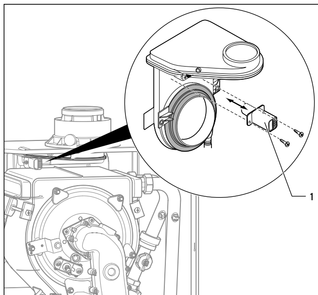
Abb. 10.4 CO-Sensor tauschen
