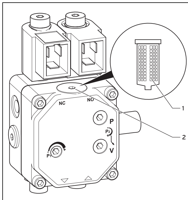
1 Ölpumpenfilter
