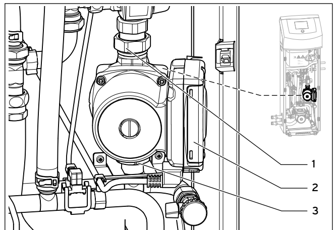
10.3 Heizungspumpe (Pufferbeladung)
