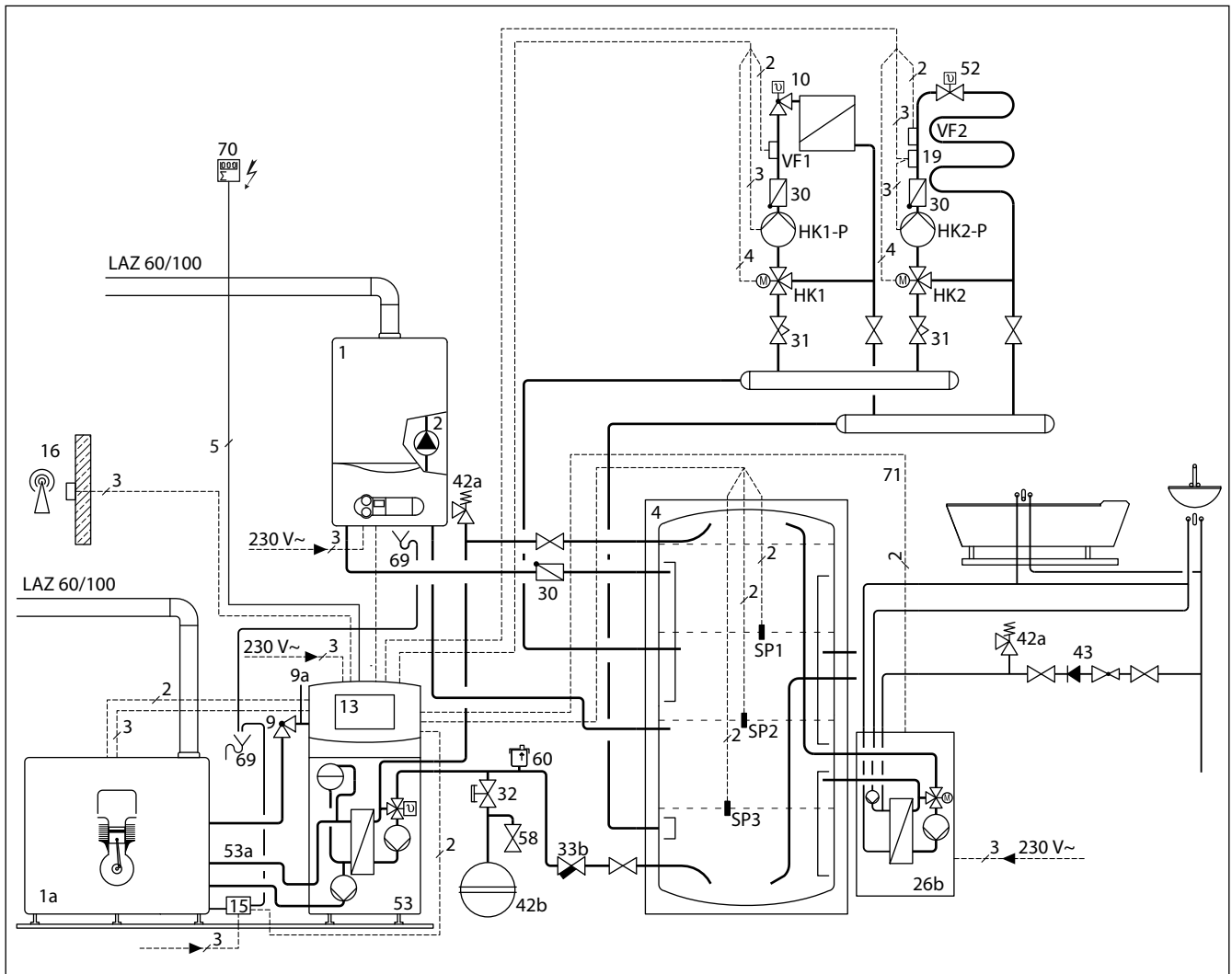
3.3 Systemschema System ecoPOWER 1.0 HS 1
