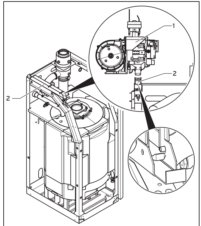
1 Brenner
