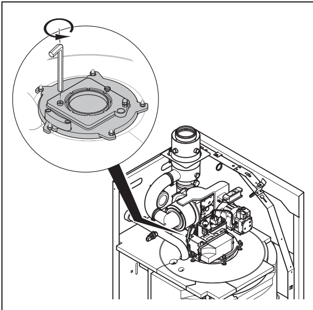
1 Brenner
