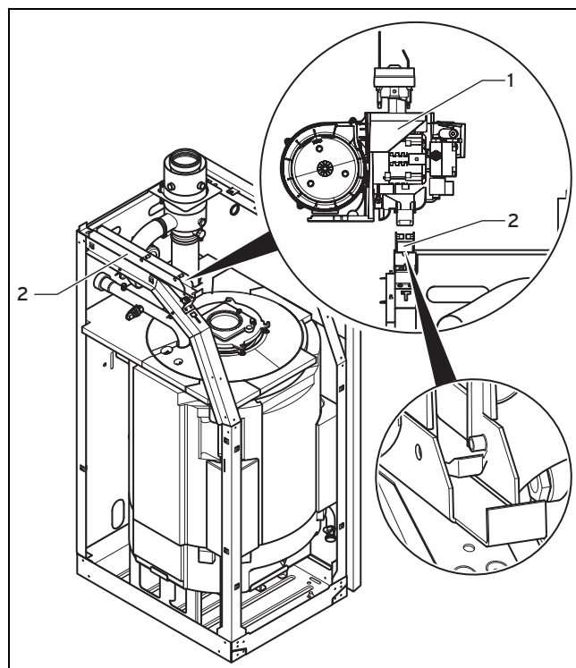
1 Brenner 2 Traverse
