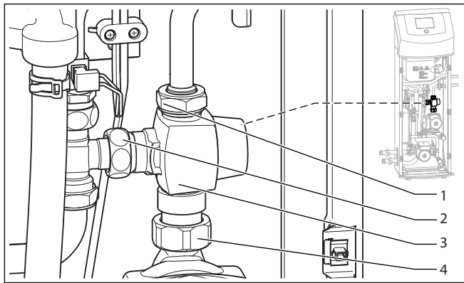
10.6 Thermostatventil
