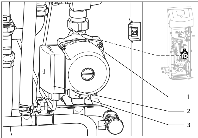
10.3 Heizungspumpe
