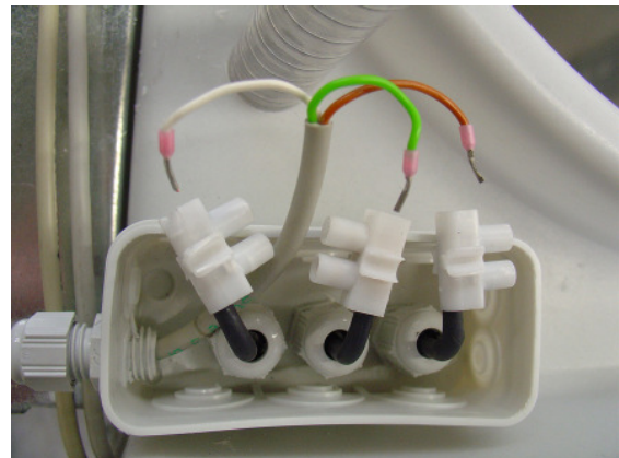
Connection level sensors
