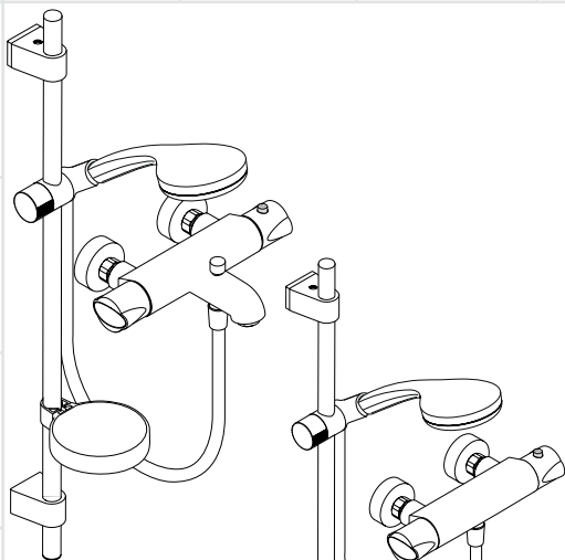
Verso Centostat Exposed Bath/ Shower Set 27291000
