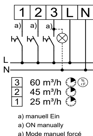
EC 60/45/25 F SS-1212
