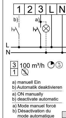
EC 100 F SS-1172
