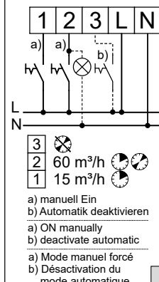
EC 60/15 NC SS-1462
