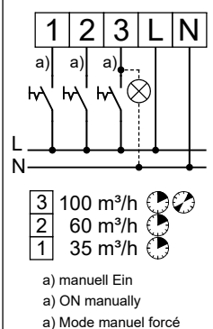
EC 100/60/35 NC SS-1170
