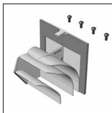
ELS-ARS Reversion kit for mounting in ELS-V... rear discharge, consisting of guide plate and 4 plastic rivets for metal nozzles.
