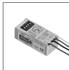
ELS-ZNI Electronic interval timer with adjustable interval and overrun times Assembly: flush-mounted box behind switch
