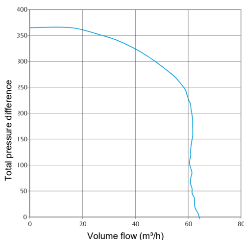
Pressure-volume characteristic curve UP-R
