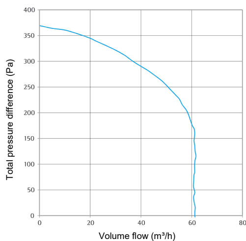
Pressure-volume characteristic curve AP
