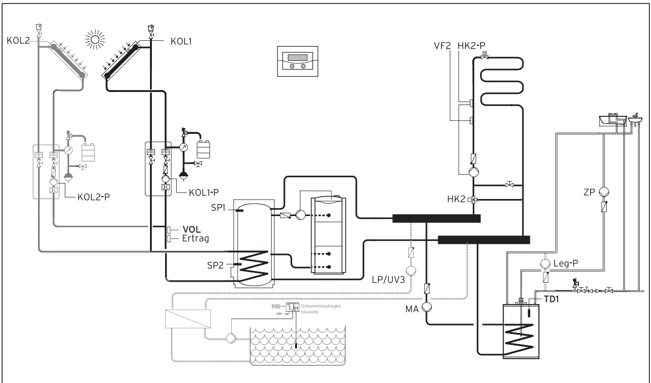
Abb. 4.23 Hydraulikplan 7
