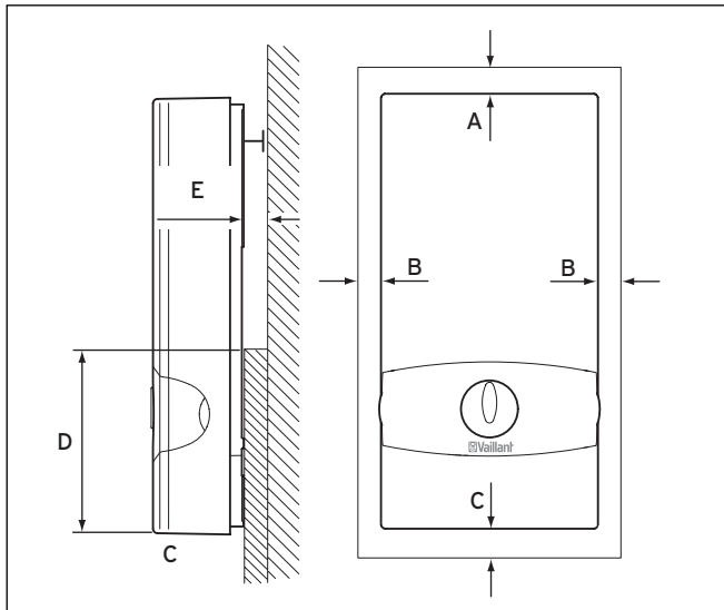
Abb. 4.2 Montagefreiräume
