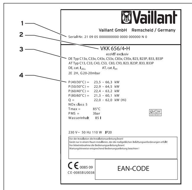
Abb. 1.1 Typenschild (Muster)
