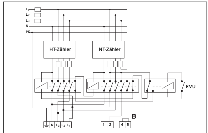
Fig. 8.4 Raccordement triphasé
