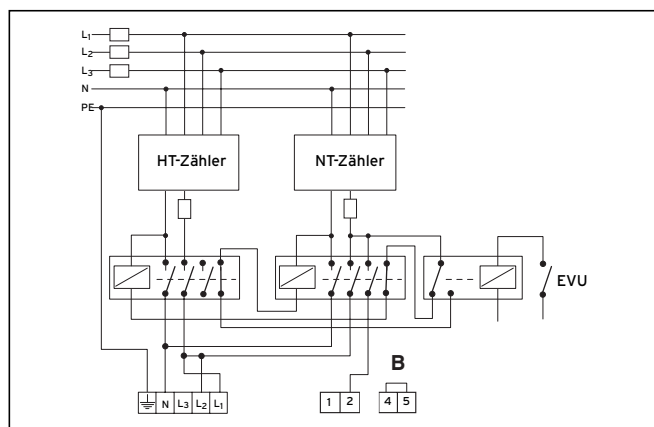
Fig. 8.2 Raccordement monophasé
