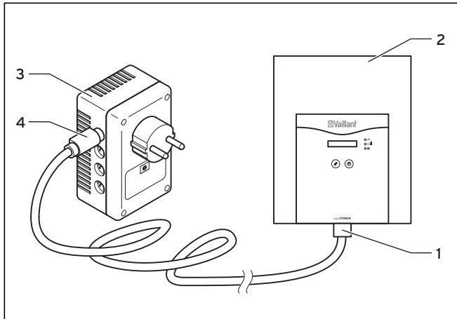
Abb. 5.1 VPI-Adapter installieren
