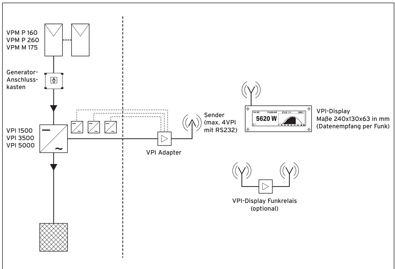
Abb. 5.1 VPI-Adapter installieren
