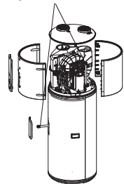
Magnesium-Anoden
