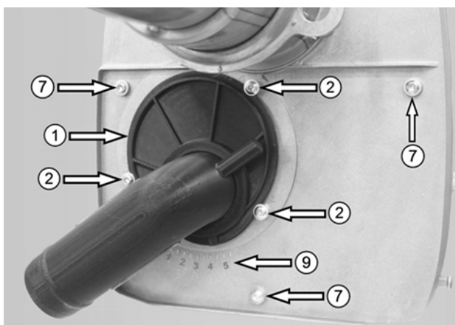
Fig. 4: Installed connection piece RLU
