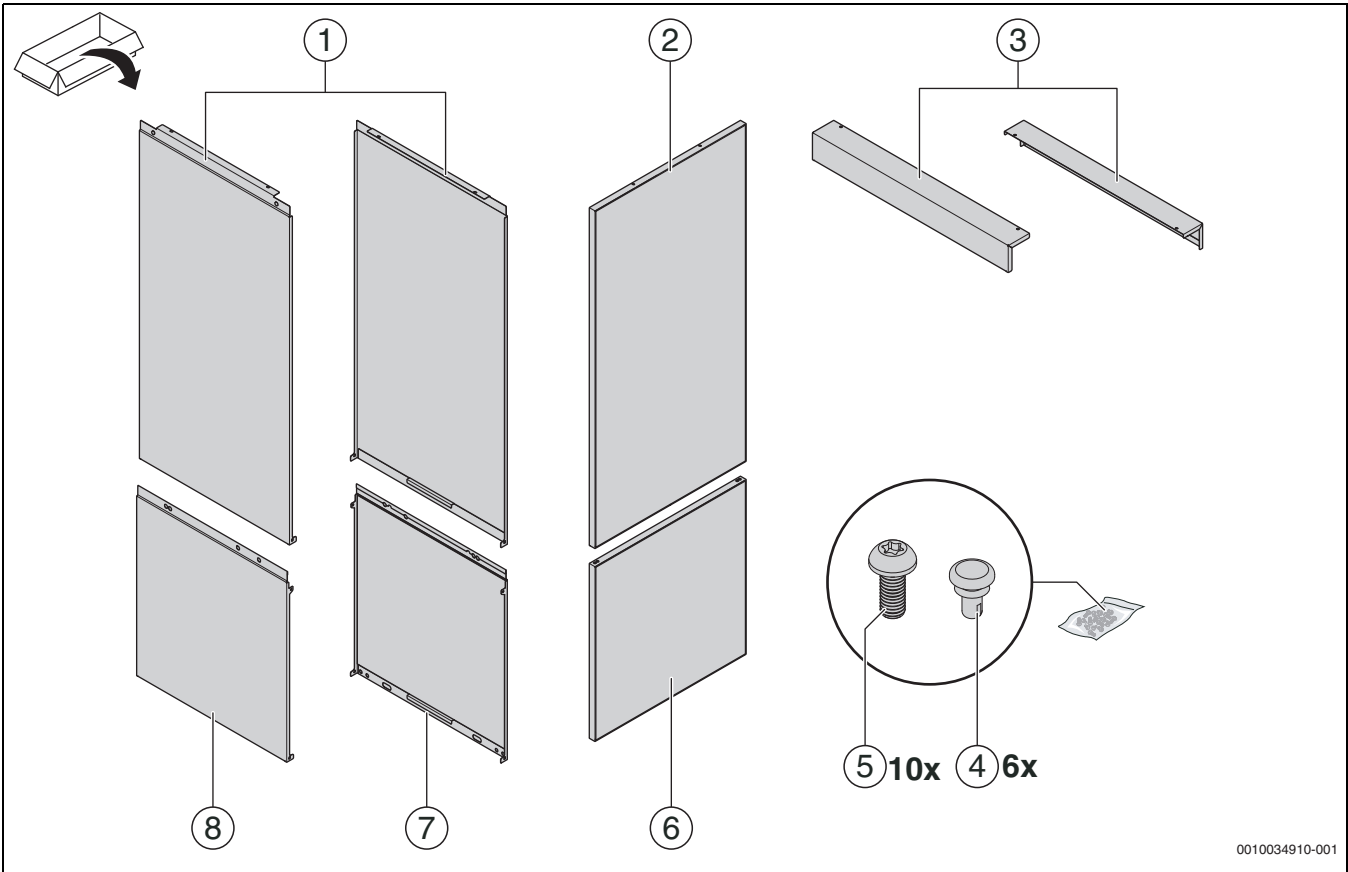
14 EWH300/EWMH300
