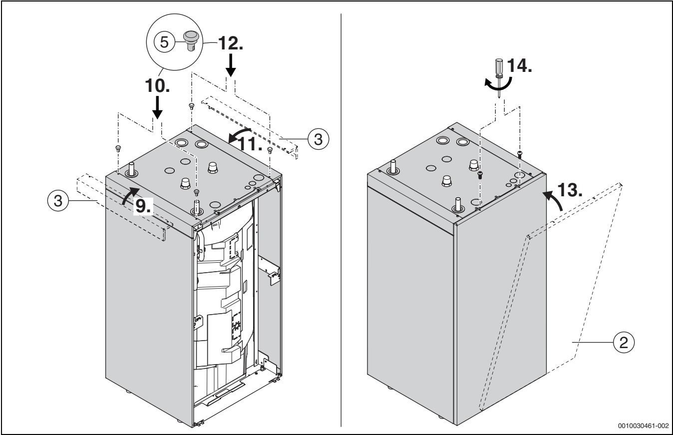
13 EWH200/EWKW250
