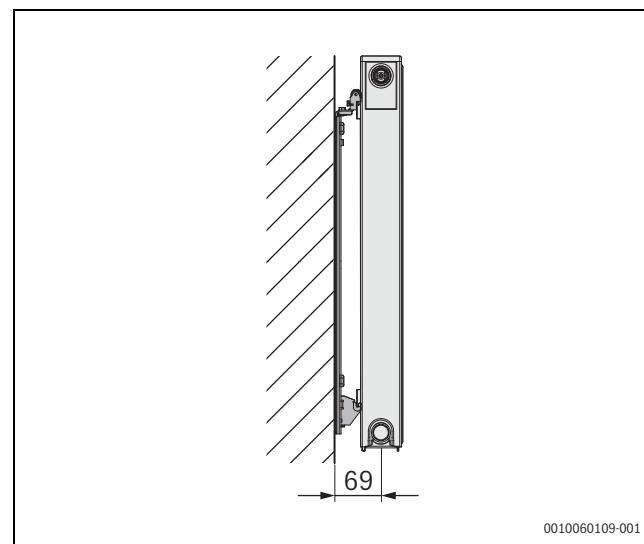
Fig. 57 Radiator bracket Type 11 for VC-, VCM-, C-Plan/Profil.2
