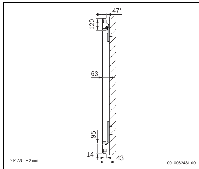
Fig. 63 Installing radiators types 10 for CV Profil/ Plan.2
