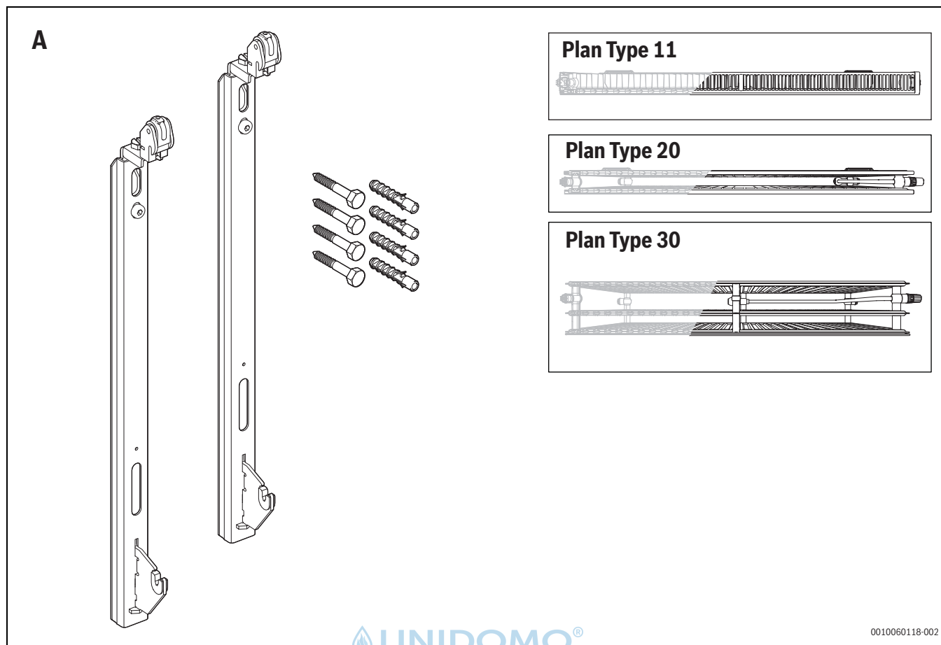
Fig. 74 Radiator bracket Type 11, 20, 30 for VC-, VCM-, C-Profil/Plan.2
