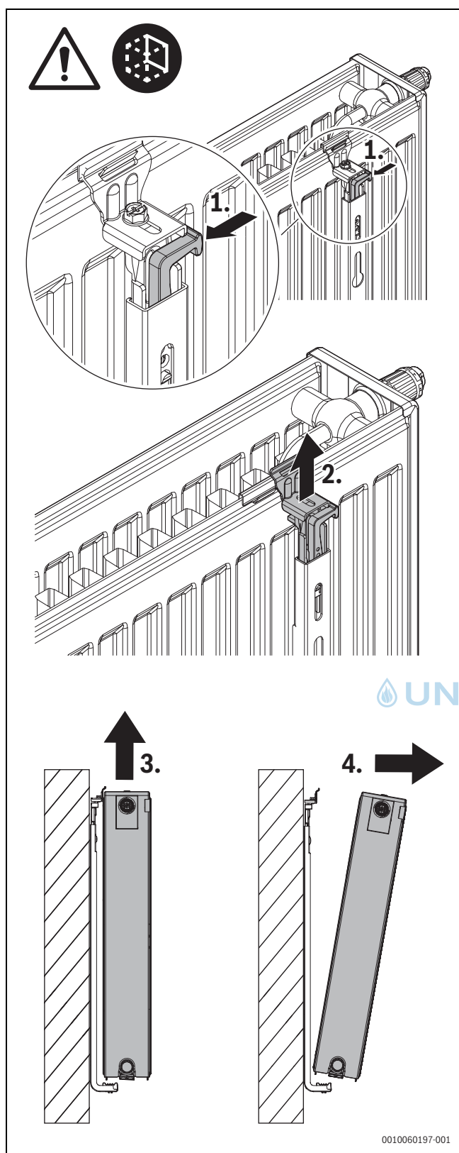
Fig. 68 Wall demounting
