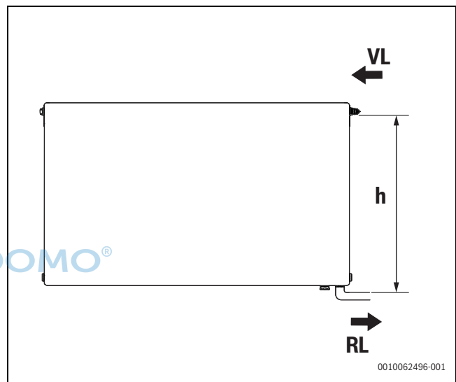
Fig. 103 Equilateral connection
