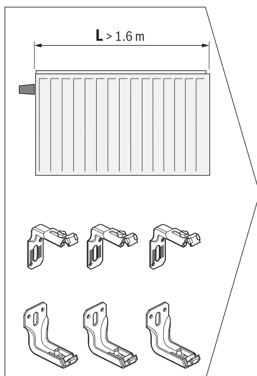
Fig. 69 Radiator bracket Type 10 for VC-, VCM-, C-Plan/Profil.2
