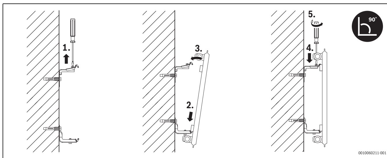
Fig. 72 Mounting the radiator to the bracket
