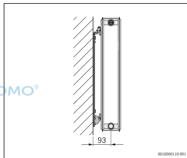
Fig. 58 Radiator bracket Type 20 for VC-, VCM-, C-Plan/Profil.2
