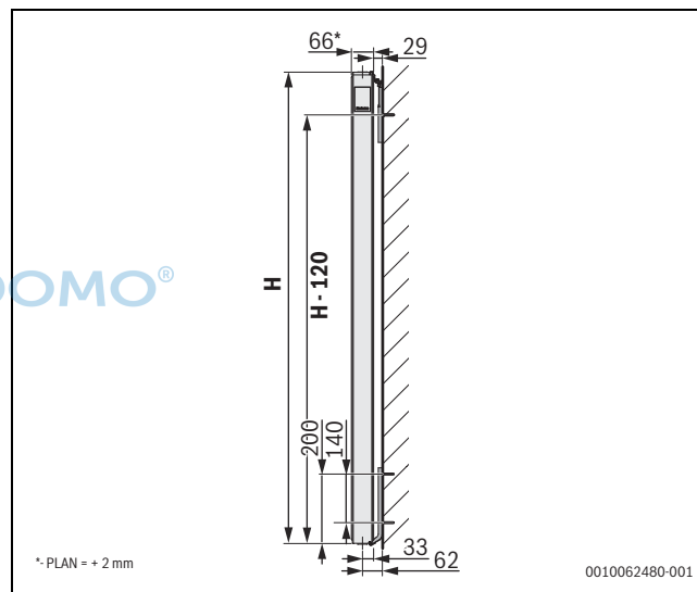
Fig. 64 Installing radiators types 20 for CV Profil/ Plan.2
