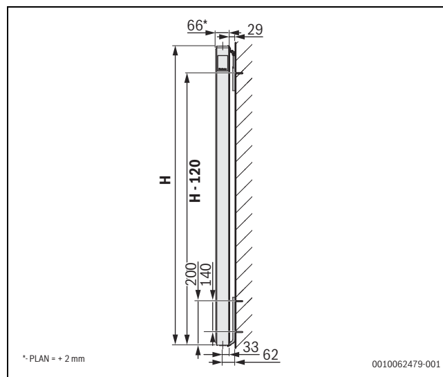
Fig. 65 Installing radiators types 21 for CV Profil/ Plan.2
