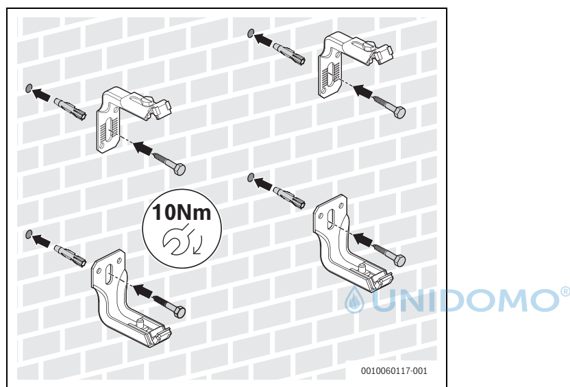
Fig. 71 Attaching the brackets to the wall
