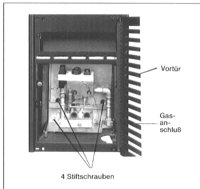
Abb. 9: Armatur SIT-Minisit-Plus
