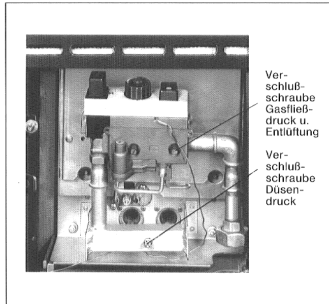
Abb. 3: Armatur SIT-Minisit-Plus
